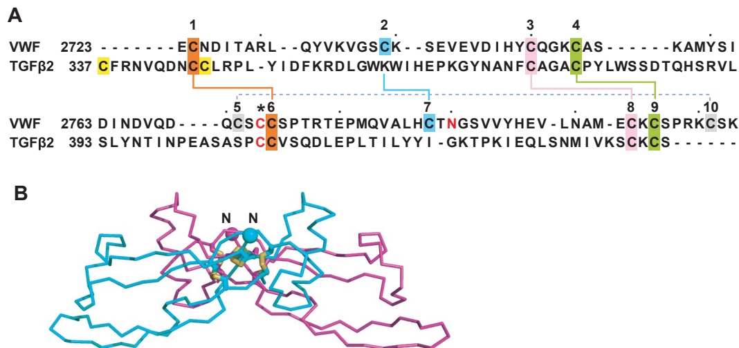
Figure 7. CTCK domain. (A) Sequence alignment of VWF CTCK domain and TGF-β2 taken from Meitinger et al. 8 Disulfides found both chemically 14 and predicted 8 or only predicted 8 are shown with solid or dashed lines, respectively, and the cysteine predicted to form the interchain disulfide is shown with an asterisk. (B) Ribbon diagram of TGF-β2 crystal structure. 40 The most N-terminal region that does not align to VWF CTCK is deleted. The new N-terminus is shown as a Cα sphere.
