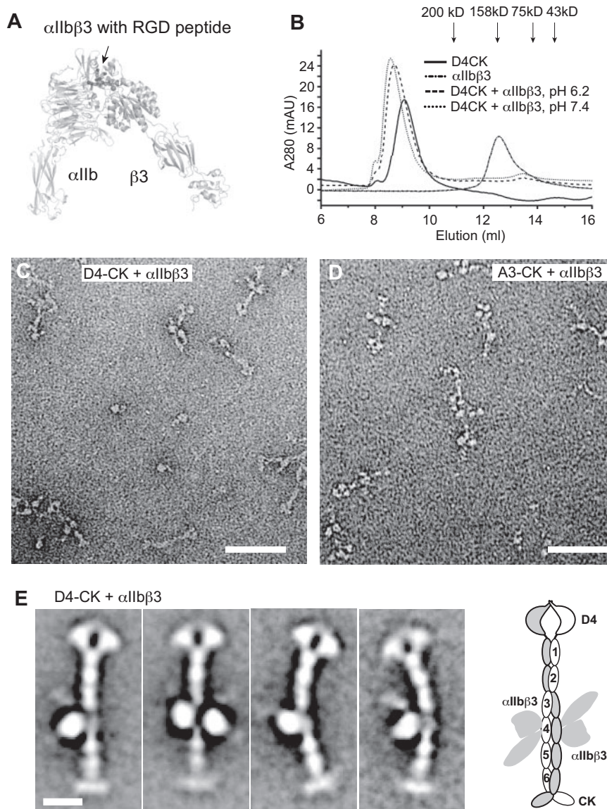
Figure 6. Binding of the integrin \alpha\text{IIb}\beta\text{3} headpiece to the VWF D4-CK fragment. (A) Overall shape of the open \alpha\text{IIb}\beta\text{3} headpiece (PDB code 2VDR and 3FCS), including the \beta -propeller and thigh domains in \alpha\text{IIb} and PSI, hybrid, \beta\text{I} , and I-EGF1 domains in \beta\text{3} subunit. Arrow shows the position of the RGD-binding site. (B) Superdex 200 gel filtration of VWF D4-CK, \alpha\text{IIb}\beta\text{3} headpiece, and their complex in 5mM \text{MnCl}_2 , 0.5mM \text{CaCl}_2 , and 0.1M \text{NaCl} and in 20mM buffer of either Bis-Tris, pH 6.2, or HEPES, pH 7.4. (C) EM image of the complex of D4-CK with the \alpha\text{IIb}\beta\text{3} headpiece at pH 6.2. (D) EM image of the complex of A3-CK with the \alpha\text{IIb}\beta\text{3} headpiece at pH 6.2. (E) Representative class averages of complex of D4-CK with the \alpha\text{IIb}\beta\text{3} headpiece. A schematic of integrin binding to VWF is shown to the right. Scale bars represent 50 nm in images and 10 nm in class averages.
