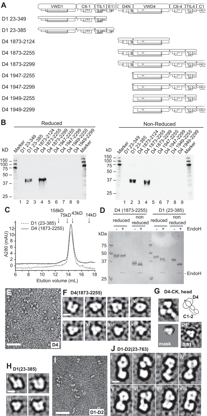
Figure 3. Expression and visualization of D assemblies. (A) D1 or D4 constructs. Cysteines are shown in vertical lines, and are connected for known and predicted disulfide bonds. (B) Expression of constructs by transient HEK293S GntI − transfectants as measured by Western blotting with anti-His tag of equal quantities of supernatants subjected to SDS 10% PAGE. (C) Superdex 200 gel-filtration of purified D1 (23-385) and D4(1873-2255) in 20mM Bis-Tris, pH 6.2, 0.15M NaCl, and 10mM CaCl 2 . Elution positions of calibration proteins are marked. (D) SDS-PAGE of D1 and D4 constructs with and without endoglycosidase H treatment stained with Coomassie blue. (E) Raw EM image of D4(1873-2255) in 20mM Bis Tris, pH 6.2, 0.15M NaCl, and 10mM CaCl 2 . (F) Representative class averages of D4(1873-2255). (G) Comparison between class averages of D4-CK head (aligned with a radius of 12 nm) and D4 (1873-2255). (H) Representative class averages of D1 (23-385) monomers at pH 6.2. (I) Raw EM image of D1-D2 (23-763) in 20mM HEPES, pH 7.4, and 0.15M NaCl. (J) Representative class averages of D1-D2. Scale bars represent 50 nm in raw images and 5 nm in class averages.
