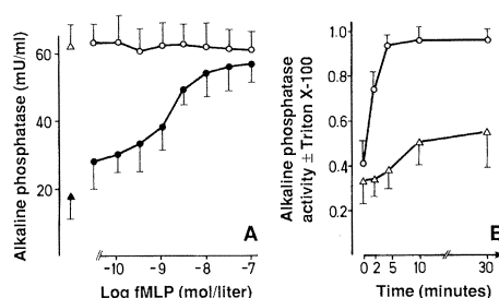
Fig. 1. Neutrophils were isolated by dextran sedimentation at room temperature and density centrifugation on Ficoll-Hypaque in the cold followed by hypotonic lysis of erythrocytes (3). (A) Purified neutrophils were incubated at 3 \times 10^7 cells per milliliter in KRP buffer (130 mM NaCl, 5.0 mM KCl, 1.27 mM \text{MgSO}_4 , 0.95 mM \text{CaCl}_2 , 5.0 mM glucose, 10 mM sodium phosphate, pH 7.4) either at 4°C ( \blacktriangle and \triangle ) or at 37°C ( \bullet and \circ ) with various concentrations of fMLP added from a 1 mM stock in ethanol. After 15 minutes, 2 volumes of ice-cold KRP was added, and the cells were sedimented by centrifugation at 200g for 8 minutes and resuspended to the original volume of 1 ml in KRP. Alkaline phosphatase was then assayed with p -nitrophenyl phosphate as substrate (23) in the absence ( \blacktriangle and \bullet ) or presence ( \triangle and \circ ) of 0.1% Triton X-100. (B) Cells were isolated as above and resuspended in KRP buffer and incubated at 3 \times 10^7 cells per milliliter at 37°C in the presence ( \circ ) or absence ( \triangle ) of 10^{-8} M fMLP. At the times indicated, the incubation was stopped and the cells were processed for determination of alkaline phosphatase in the presence or absence of 0.1% Triton X-100 as described above. Results are the mean of three experiments. Bars indicate 1 SD.
