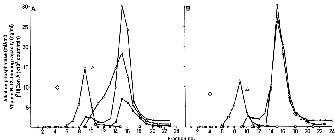
Fig. 2. Neutrophils, 1.2 \times 10^9 isolated as in Fig. 1, were resuspended at 4^\circ\text{C} in KRP to a concentration of 5 \times 10^7 cells per milliliter. Fifty microliters of ^3\text{H} -labeled acetylated Con A (Amersham, 60 Ci/mmol, 50 \mu\text{Ci}/\text{ml} ) was added and the suspension was incubated at 4^\circ\text{C} for 10 minutes, and then divided in two. The cells were sedimented by centrifugation and resuspended to a concentration of 5 \times 10^7 cells per milliliter in KRP. One sample was kept at 4^\circ\text{C} (A), the other was incubated at 37^\circ\text{C} with 10^{-8}\text{M} fMLP (B). After 15 minutes, 2 volumes of ice-cold KRP containing 10 mM diisopropyl fluorophosphate was added to both samples, and these were further incubated on ice for 10 minutes. The cells were then sedimented by centrifugation and resuspended in 15 ml of relaxation buffer [100 mM KCl, 3 mM NaCl, 1 mM adenosine triphosphate (ATP)Na 2 , 3.5 mM MgCl 2 , 10 mM 1,4-piperazinediethanesulfonic acid (Pipes), pH 7.3] containing 0.5 mM phenylmethylsulfonyl fluoride (PMSF) and subjected to nitrogen cavitation (3). Ten milliliters of the postnuclear supernatants ( S_1 ) [protein concentration
