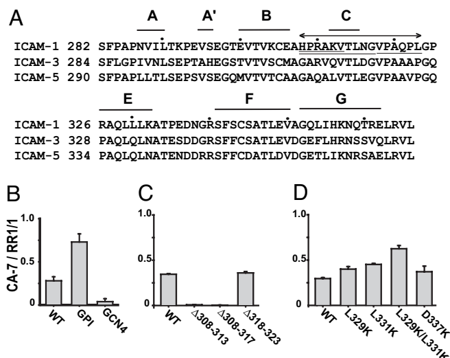
Fig. 5. Secondary structure of D4 and the effect of mutations on monomer-dimer equilibrium on the cell surface. (A) Secondary structure of D4 of ICAM-1 and alignment with D4 of ICAM-3 and ICAM-5. Every 10th residue is marked with a dot. The 16 residues disordered in dimeric ICAM-1 are indicated by a line with two arrowheads. The three deleted regions are underlined. (B–D) The proportion of monomeric ICAM-1 on wild-type ICAM-1, GPI-ICAM-1, and GCN4–293T transfectants as measured by immunofluorescent flow cytometry and the ratio of CA7 (monomer specific) to RR1/1 (conformation-independent) antibody staining. (B) Comparisons of GPI-ICAM-1 and GCN4-ICAM-1 mutants. (C) Comparison of deletion mutants. (D) Comparison of point mutants.
