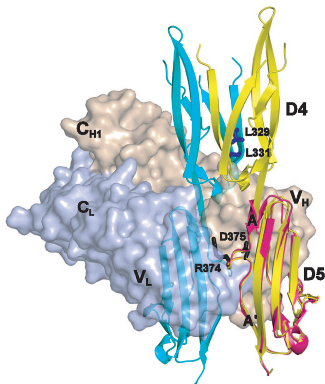
Fig. 4. The CA7 Fab binding site in D5. CA7 Fab is shown as a surface representation colored in wheat (heavy chain) and light blue (light chain) bound to monomeric D5 shown as a magenta ribbon, with indicated side chains in the AA loop at the center of the epitope as black sticks. Dimeric D4 and D5 are shown as ribbons with a cyan monomer and a yellow monomer superimposed on monomeric D5. The inward-pointing Leu residues of \beta -strand E of the cyan monomer are shown as blue sticks.
