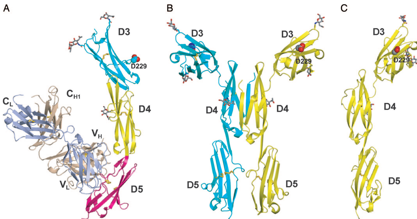
Fig. 1. Ribbon diagrams of ICAM D3–D5 crystal structures. (A) Monomeric ICAM-1 D3–D5 complexed with CA7 Fab. (B) The dimeric ICAM-1 D3–D5 structure (8). (C) The monomeric ICAM-1 D3–D5 structure with CA7 Fab omitted, shown in the same orientation as the right monomer of dimeric D3–D5 in B, after superposition on D4. The side chain of the key \alpha_M\beta_2 binding residue in D3, Asp-229, is shown with large spheres. The Fab light and heavy chains are shown in light blue and wheat, respectively. Glycans are drawn in stick with red oxygens and gray carbons. Disulfide bonds are drawn as gold sticks.
