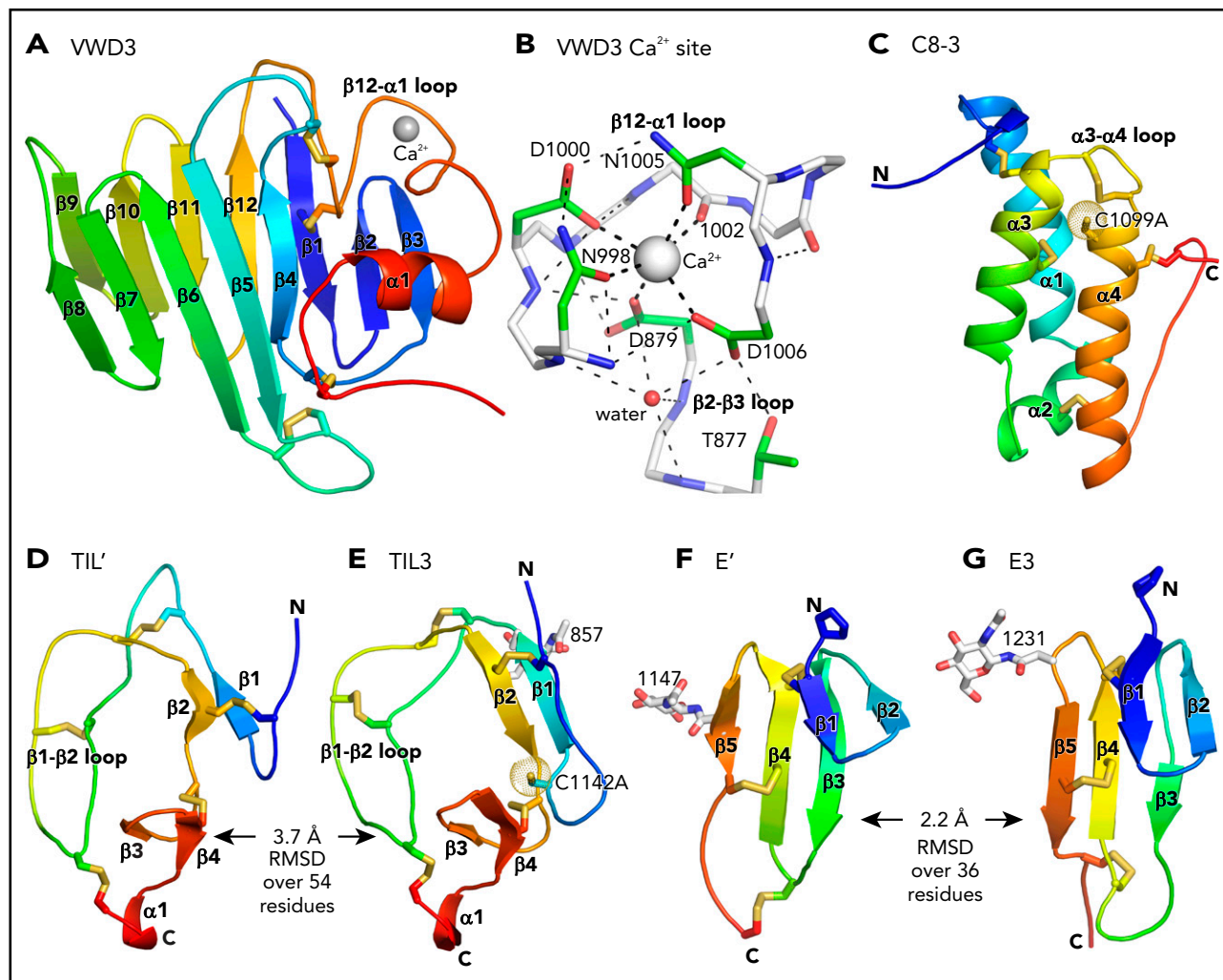
Figure 3. Structure of D assembly modules. (A,C-G) Each module is shown rainbow colored to trace the path the polypeptide takes to create the fold, from N terminus (blue) to C terminus (red). (B) The \text{Ca}^{2+} -binding site. Mainchain carbons are shown in white, with sidechain carbons in green. \text{Ca}^{2+} and a water oxygen are shown as spheres. Coordination bonds to the \text{Ca}^{2+} and hydrogen bonds are shown as thick and thin dashed lines, respectively. Other representations are as in Figure 1. Superposition of TIL domains required the Deep Align server 27 ; E modules were superimposed with PyMol. Superimposed structures are shown separated horizontally on the page. Structural differences between modules are shown as root mean square deviation of \text{C}\alpha atoms.
