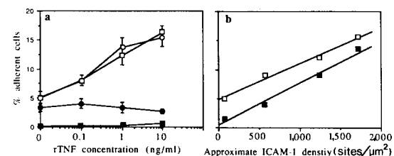
Figure 5. Effect of TNF treatment on JY adhesion and ICAM-1 expression. HUVEC were grown to confluence in 96 well plates and were incubated with the indicated concentration of rTNF for 16 h. Adhesion of ^{51}\text{Cr} JY cells was measured as described in methods. Binding of [ ^{125}\text{I} ]ICAM-1 mAb was determined in parallel. (a) (Open squares) control mAb; (open circles) anti-HLA A,B; (solid squares) LFA-1 mAb; (solid circles) ICAM-1 mAb. (b) Adhesion data same as in a. (Solid squares) binding inhibitable by LFA-1 mAb; (solid circles) binding inhibitable by ICAM-1 mAb. Density is approximated assuming all ICAM-1 is expressed on an area with the dimension of the well (0.28 cm 2 ). Similar results were obtained in two other experiments.
