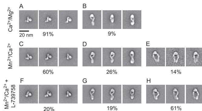
FIGURE 2. Two-dimensional class averages of intact \alpha_{IIb}\beta_3 . Representative class averages of DDM-solubilized \alpha_{IIb}\beta_3 in Ca^{2+}/Mg^{2+} (A and B), Mn^{2+}/Ca^{2+} (C–E), and Mn^{2+}/Ca^{2+} with L-739758 (F–H) are shown. The percentage of the particles represented by bent (A, C, and F), extended-closed (B, D, and G), and extended-open (E and H) is shown below the panels.
