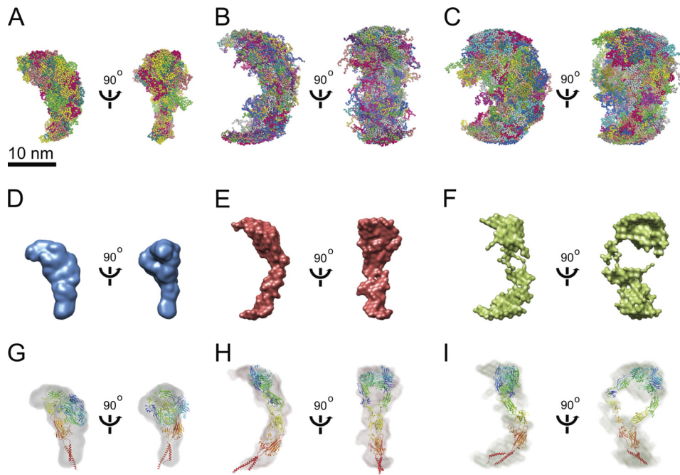
FIGURE 4. SAXS ab initio models. SAXS ab initio models of \alpha_{IIb}\beta_3 in \text{Ca}^{2+}/\text{Mg}^{2+} (A, D, and G), \text{Mn}^{2+}/\text{Ca}^{2+} (B, E, and H), and \text{Mn}^{2+}/\text{Ca}^{2+} with L-739758 (C, F, and I) are shown. A–C, 20 superimposed bead models calculated by GASBOR (42). D–F, envelope models of the averaged bead models calculated by DAMAVER (43) scaled at 4 \times 10^5 \text{ \AA}^3 in Chimera (44). G–I, envelope models of \alpha_{IIb}\beta_3 docked with atomic models by cross-correlation maximization in Chimera (44). G, the full \alpha_{IIb}\beta_3 ectodomain crystal structure (Protein Data Bank code 3FCS) with modeled transmembrane domains is shown in ribbon diagram. H and I, the extended atomic models were generated by manually changing the bends in the \alpha and \beta subunit knees (supplemental Fig. 3, B and C) to resemble SAXS envelope models.
