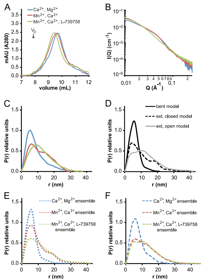
FIGURE 3. Tracking \alpha_{IIB}\beta_3 extension by size exclusion chromatography and SAXS. \text{Ca}^{2+}/\text{Mg}^{2+} buffer conditions are shown in blue, \text{Mn}^{2+}/\text{Ca}^{2+} buffer conditions are shown in red, and \text{Mn}^{2+}/\text{Ca}^{2+} and L-739758 buffer conditions are shown in green. A , Superdex 200 gel filtration runs of \alpha_{IIB}\beta_3 in TBS, pH 7.4 with a 1 \times CMC of DDM. Note the lack of aggregated material in the void volume ( V_0 ). B , x-ray solution scattering curves of 2.3 mg/ml \alpha_{IIB}\beta_3 in TBS, pH 7.4 with a 1 \times CMC of Triton X-100. C , distance distribution plot of data in B . D , distance distribution plot of atomic models of \alpha_{IIB}\beta_3 in the bent (black line), extended-closed (dashed line), and extended-open (gray line) conformations. E , distance distribution plots of modeled ensembles of \alpha_{IIB}\beta_3 based on EM in \text{Ca}^{2+}/\text{Mg}^{2+} with 91% bent and 9% extended-closed (blue dotted line); \text{Mn}^{2+}/\text{Ca}^{2+} with 60% bent, 26% extended-closed, and 14% extended-open (red dotted line); and \text{Mn}^{2+}/\text{Ca}^{2+} and L-739758 with 20% bent, 19% extended-closed, and 61% extended-open (green dotted line). F , distance distribution plots of modeled ensembles of \alpha_{IIB}\beta_3 by least square fitting to experimental data in \text{Ca}^{2+}/\text{Mg}^{2+} with 50% bent and 50% extended-closed (blue dashed line); \text{Mn}^{2+}/\text{Ca}^{2+} with 20% bent, 5% extended-closed, and 75% extended-open (red dashed line); and \text{Mn}^{2+}/\text{Ca}^{2+} and L-739758 with 15% bent and 85% extended-open (green dashed line). mAU, milliabsorbance units; ext, extended.
