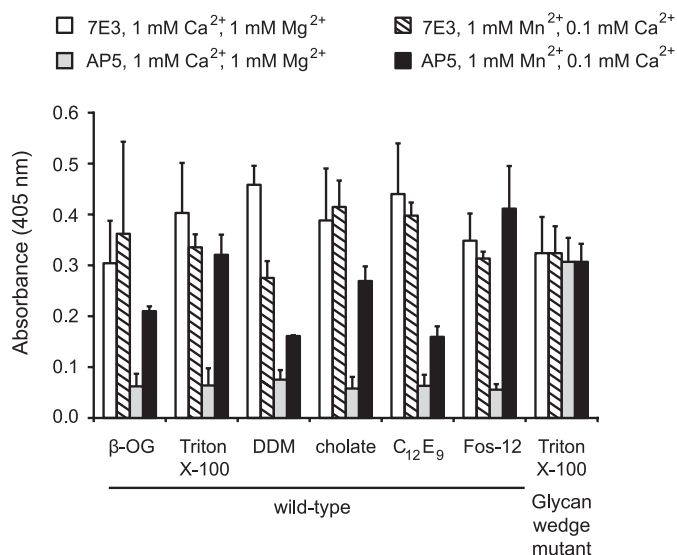
FIGURE 1. Mn^{2+} -induced activation increases LIBS exposure of detergent-solubilized integrin. ELISA-based assay was used to detect the amount of total and active \alpha_{IIb}\beta_3 in Ca^{2+}/Mg^{2+} (white and gray bars) and Mn^{2+}/Ca^{2+} (striped and black bars) in various detergents. \alpha_{IIb}\beta_3 was captured using mAb AP3 (conformation-independent anti- \beta_3 ) and assayed for the total amount of receptor using 7E3 (white and striped bars), a conformationally independent anti- \beta_3 mAb, and for the amount of active receptor using AP5 (gray and black bars), a LIBS mAb detecting the plexin-semaphorin-integrin domain. The high affinity, N-glycan wedge mutant that introduces an N-glycosylation site at Asn-303 was used as a control for maximum AP5 binding. Error bars are 1 S.D. with a sample size of n = 4 . \beta -OG, octyl \beta -D-glucopyranoside.
