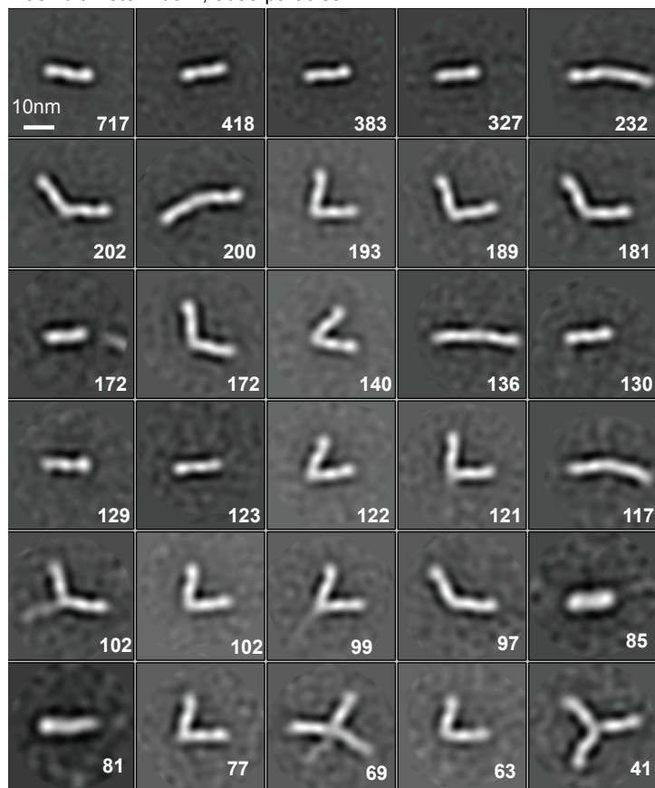
B pH 5.0, \beta -DDM, 26 h at 37°C; box diameter 410 Å, mask diameter 400 Å, 5693 particles
