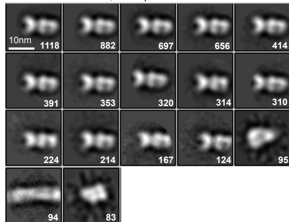
C pH 1.5, \beta -DDM, 26 h at 37°C; box diameter 213 Å, mask diameter 200 Å, 6456 particles
