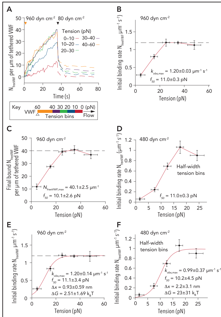
Figure 2. Tension-regulated VWF self-association. (A) Average time course of VWF ( 10 \mu\text{g mL}^{-1} ) binding to single tethered VWF concatemers at 960 \text{ dyn cm}^{-2} . Curves show association (solid lines) and dissociation (dashed lines) at 80 \text{ dyn cm}^{-2} and are color coded by tension bin as shown in the key (the triangle shows the tether point). Data are averaged from 62 tethered VWF molecules used in Figure 1C-E that are large enough to include a 40-to-60 pN tension bin at 960 \text{ dyn cm}^{-2} . (B) Initial VWF binding rate and (C) final bound density of VWF from data in panel A. In panels B and C, the maximum binding rate and total binding density are estimated as the average of the values in the 20-to-30 and 30-to-40 pN bins. The force at half-maximal binding, f_{50} , was determined as the intercept of the half maxima with the lines drawn through the data points on either side of the half maxima. (D) Initial binding rate of VWF ( 10 \mu\text{g mL}^{-1} ) at 480 \text{ dyn cm}^{-2} using smaller (5 pN) tension bins. In panels B-D, red lines connect neighboring points. (E-F) Fits of the data in panels B and D to a 2-state model (red lines) in which the observed initial binding rate k_{\text{obs}} = k_{\text{obs,max}} / (1 + \exp((\Delta G - f \cdot \Delta x) / k_B T)) , where k_{\text{obs,max}} is the maximum observed initial binding rate, \Delta G is the free energy difference between the 2 states (fast binding and slow or no binding), and \Delta x is the displacement along the force f direction between the 2 states. Data in panels A-F are from the same set of tethered VWF concatemers. In panels B-D, error bars represent standard deviation. In panels E-F, error bars represent standard deviation for tension and 95% confidence intervals for the other variables.
