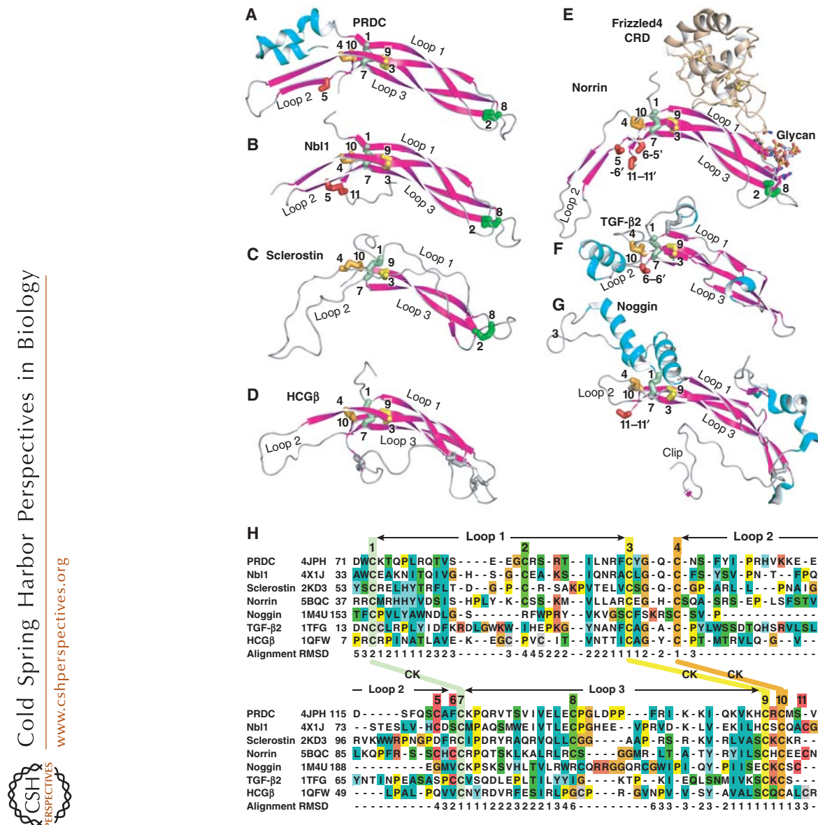
Figure 11. Structural alignment of Dan family monomers to cystine knot (CK) growth factor (CKGF) superfamily representatives with similar monomer–monomer orientations. (A–G) CKGF monomers in cartoon with \alpha -helices in cyan and \beta -strands in magenta. Disulfides are shown in stick and are color-coded with their cysteines numbered as in panel H . Cysteines in intermolecular disulfides are indicated by showing the partner Cys in the other monomer with its number preceded by a dash and followed by a hyphen. All monomers but sclerostin are from dimeric structures. A frizzled domain and glycan cocrystallized with norrin are shown in cartoon and stick, respectively. Monomers are in identical orientations, and aligned in two columns. (H) Structure-based sequence alignment. Cysteines disulfide-bonded to one another are in identical colors, except those that participate in interchain disulfides in some families and intrachain disulfides in others (positions 5, 6, and 11) are shown in red. Disulfides unique to particular families are shown in thinner silver stick and colored silver in panel H . Other residues are colored according to ClustalX. CK disulfides are labeled between the two rows of the alignment and link Cys residues distant in sequence; the three long loops between CK disulfides are also marked. (Legend continues on following page.)
