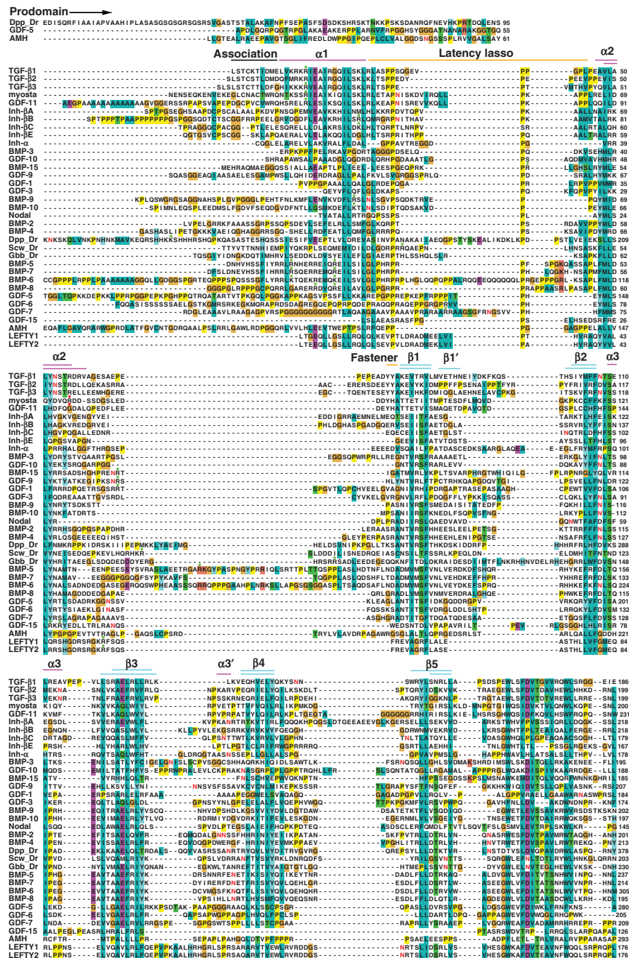
Figure 1. Sequence alignment of the transforming growth factor β (TGF-β) family. Sequences were aligned with MAFFT (Katoh and Standley 2013), as described (Shi et al. 2011), with slight structural realignment of TGF-β1 and bone morphogenetic protein (BMP)-9 procomplexes (Mi et al. 2015). Structure elements of pro-TGF-β1 (Shi et al. 2011) and pro-BMP-9 (Mi et al. 2015) are labeled and shown as colored lines ( upper and lower lines , respectively). ( Legend continues on following page. )
