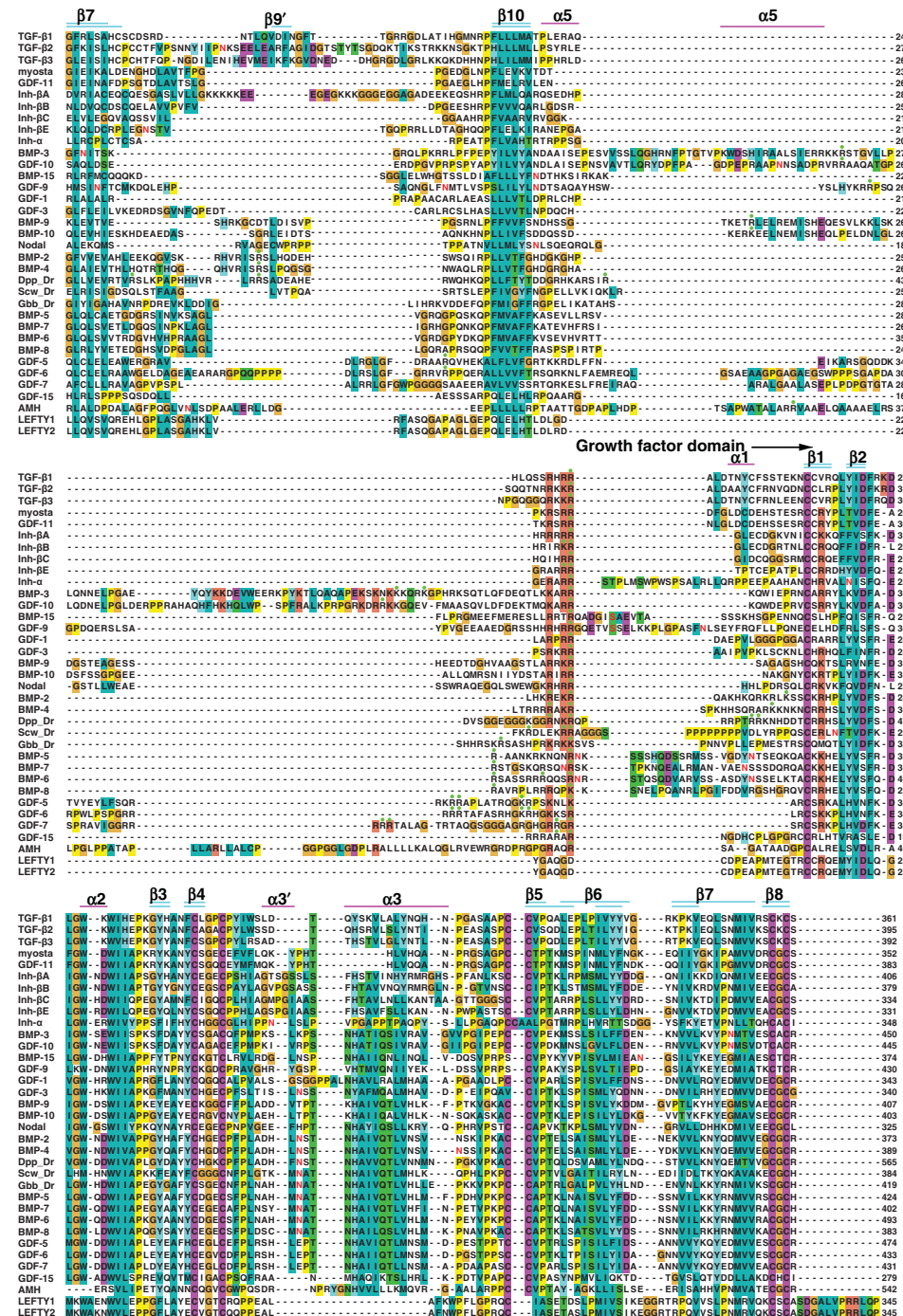
Figure 1. (Continued) Potential proprotein convertase (PC) and tolloid cleavage sites are marked with green and red circles, respectively. Potentially N-glycosylated asparagines in all family members and known phosphorylated serines in mature BMP-15 and growth and differentiation factor 9 (GDF-9) (Tibaldi et al. 2010) are shown in bold red. All 33 human TGF- \beta family polypeptides are shown, except BMP-8B; the almost identical BMP-8A is shown as BMP-8. Three well-characterized Drosophila melanogaster BMPs are included: Decapentaplegic (Dpp), Screw (Scw), and Glass bottom boat (Gbb). Closely related family members appear in adjacent rows.
