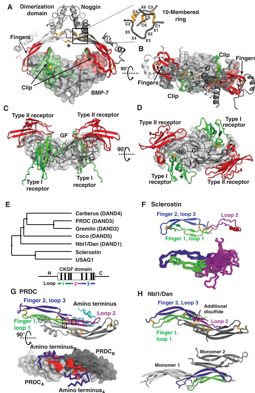
Figure 12. The bone morphogenetic protein (BMP) modulator noggin, members of the Dan family, and sclerostin. (A) Noggin binds BMPs (PDB 1M4U [Groppe et al. 2002]) in a clamp-like manner with the fingers of its cystine knot (CK) growth factor (CKGF) domain (red) blocking type II receptor binding, and a peptide segment termed clip (green) shielding the type I receptor epitopes. Hydrophobic Pro35 of noggin, engaging in the knob-into-hole interaction motif is shown as a gold sphere. The noggin dimer is formed by interactions between the \alpha -helical dimerization domains and stabilized by an intermolecular disulfide bond (asterisk). Disulfides are shown with gold sticks and the CK motif (box) is shown in detail. (B) As in A but viewed down the dyad axis of the noggin and GF dimers. (C and D) A prototypical BMP ligand-receptor complex, with type I and type II receptors as green and red ribbons, respectively, and the GF dimer as gray surface (PDB 2H64 [Weber et al. 2007]) shown in similar orientations as in A and B. (Legend continues on following page.)
