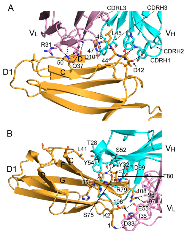
FIGURE 3. MAdCAM-Fab interfaces. A, MAdCAM complex with 10G3 Fab. B, MAdCAM complex with PF-547659 Fab. Heavy chain is cyan; light chain is pink, and MAdCAM D1 is orange. Side chains and main chain atoms in the interfaces and the integrin binding loop of MAdCAM are in stick. MAdCAM Gly residues 40 and 46 have \text{C}\alpha spheres. Dashed lines show hydrogen bonds across the interfaces.
