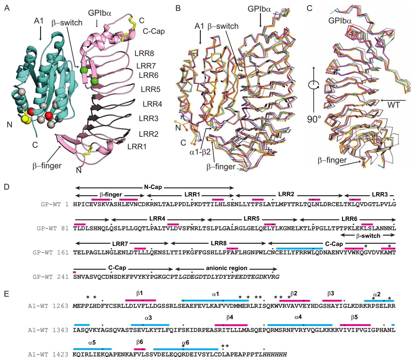
FIGURE 1. The VWF A1-GPIIb \alpha complex. A, overall structure in a schematic diagram. A1 (cyan) has a central \beta -sheet that interacts with GPIIb \alpha (pink) by forming an extended \beta -sheet with the GPIIb \alpha \beta -switch. A single disulfide bond in A1 and three disulfide bonds in GPIIb \alpha are shown in yellow stick form. VWD type 2B mutations locate near the A1 termini distant from the GPIIb \alpha interface and are shown as \alpha spheres in red (R1306Q and I1309V type 2B mutations used in this study), silver (other 2B mutations), and yellow (Y1271C and C1272R mutations used here). PT-VWD mutations locate in the GPIIb \alpha \beta -switch region (green \alpha spheres for the G233V and M239V mutations used here). GPIIb \alpha LRR2 to -4, shown not to bind to A1 in previous crystal structures but to be important for ristocetin and shear-induced binding to VWF (15), are shown in gray. B and C, previous and current A1-GPIIb \alpha complexes superimposed on A1 and shown as \alpha ribbons. Magenta, A1/VWD2-GPIIb \alpha /VWD2; orange, A1/SS-GPIIb \alpha /VWD2, chains E and F; yellow, chains G and H; cyan, A1/VWD1-GPIIb \alpha /VWD1 (12), PDB code 1M10; silver, A1/WT-GPIIb \alpha /WT (44), PDB code 1S0Q. C, the same superposition, rotated 90° to show the A1-binding face of GPIIb \alpha with A1 removed. D and E, sequences with secondary structure overlined, GPIIb \alpha regions marked, and decadal residues dotted. Regions present in constructs but disordered in crystals are in italic type. PT-VWD mutations used here and known VWD type 2B mutations are marked with asterisks.
