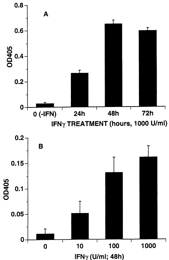
FIG. 2. Time course and concentration dependence of IFN \gamma -induced cell surface ICAM-1 expression on T84 cells
