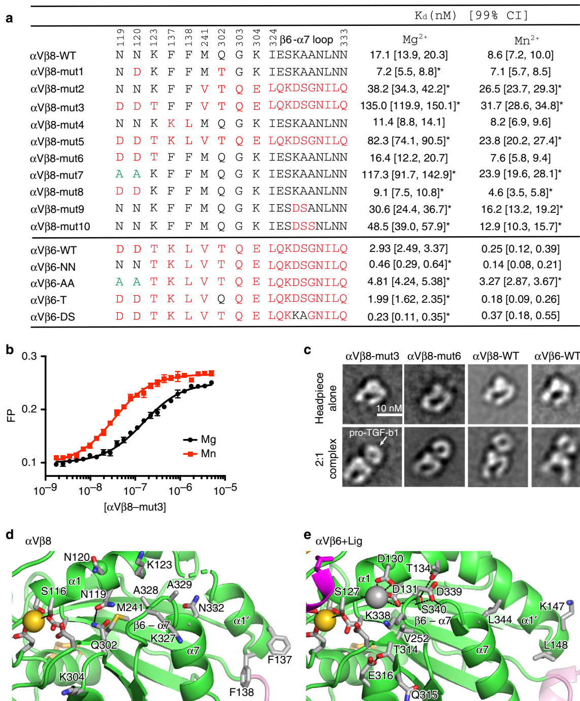
Fig. 7 Regulation of ligand-binding affinity by atypical and typical residues in \alpha V \beta 8 and \alpha V \beta 6. a Mutations corresponding to sequence exchanges between \alpha V \beta 8 (black) and \alpha V \beta 6 (red) and effect on affinity for FITC-labeled TGF- \beta 3 ligand peptide (GRGDLRKK) in presence of Mg^{2+} and Mn^{2+} . K_D and [99% confidence interval] values were determined by fluorescence polarization and fits using the NonLinearModelFit function of Mathematica (Wolfram, Champaign, IL) of all data from measurements in triplicate of two different experiments done in different months. As in statistical models for determining p values, the fit assumes that errors are independent and normally distributed. The reported fit minimizes the sum of the squared errors. If two values have 99% confidence intervals that do not overlap, then the two values by definition have <1% chance of being different by chance alone, that is, the p value is <0.01. Therefore, mutant K_D values with confidence intervals that do not overlap with those of WT are significantly different ( p < 0.01 ) and are asterisked. b Representative fluorescence polarization (FP) of \alpha V \beta 8-mut3 from one triplicate experiment (average \pm s.d) with fit (line). Source data for a , b are provided as a Source Data file. c Representative negative stain class averages of mutant or WT integrin headpieces alone (upper panels) or complexed with pro-TGF- \beta 1. Representative 2:1 pro-TGF- \beta 1:integrin class averages are shown. The WT integrin class averages shown for comparison are previously published 14 . d , e Residues in regions of \beta 1 domain allosteric with unusual properties in \alpha V \beta 8 ( d ) are compared to counterparts in \alpha V \beta 6 ( e ).
