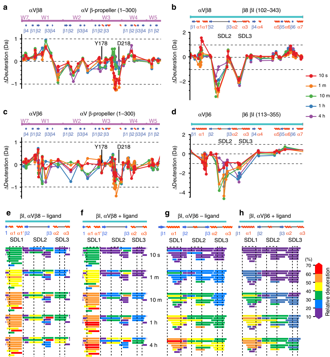
Fig. 6 Effect of ligand binding on deuterium exchange. a–d Differences in HDX with and without saturating concentrations of TGF- \beta 1 ligand peptide G 213 RRGDLATHIG 223 for \alpha V\beta 8 and \alpha V\beta 6 are shown for each peptide plotted at the midpoint of its sequence position for a portion of the \beta -propeller domain and the entire \beta I domain. The equation for subtraction was (D_{\text{liganded}} - D_{\text{unliganded}}) . Differences > 1 Da (dashed lines) are considered meaningful. All HDX data are presented in Supplementary Figs. 1 and 2. e–h Details of the ligand-binding region of the \beta I domain. Exchange in each peptide is colored according to the key.
