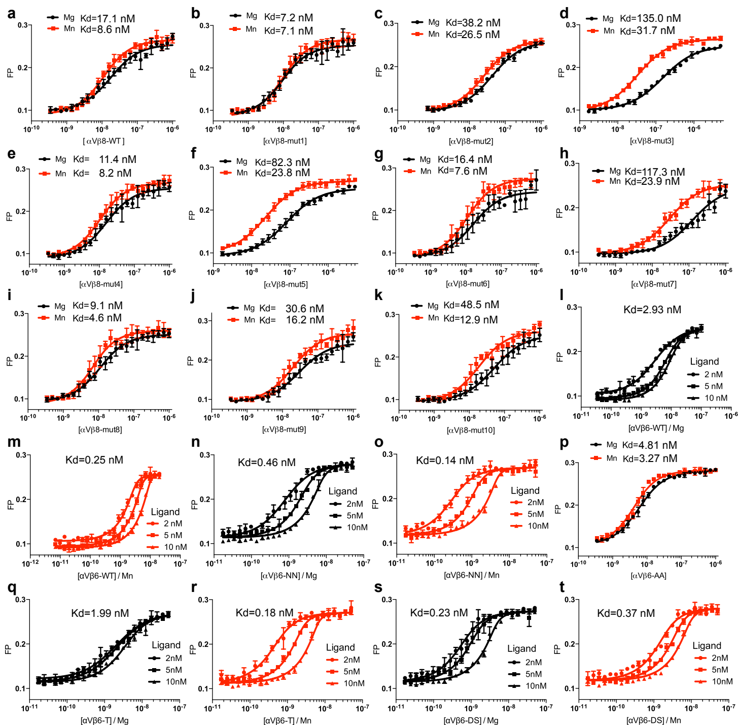
Supplementary Figure 3. Representative affinity measurements. (a-t). Data points and fitting curves for FP measurements. Data points were fit to a ligand-depletion model in GraphPad Prism as previously described 1 . For \alpha V\beta 8 wild type and mutants, a single probe concentration was used for all measurements. For \alpha V\beta 6 wild type and mutants except for \alpha V\beta 6 -AA, three different probe concentrations were used to more accurately determine the concentration of input ligand and better account for the effect of high-affinity binding on ligand depletion. Representative fluorescence polarization (FP) from one of two triplicate experiments (average \pm s.d) with fit (line) is shown for each mutant. The inset K_D values were determined using the NonLinearModelFit function of Mathematica (Wolfram, Champaign IL) using all data from measurements in triplicate of two different experiments done in different months. The fit assumes that errors are independent and normally distributed and minimizes the sum of the squared errors. Source data are provided as a Source Data file.
