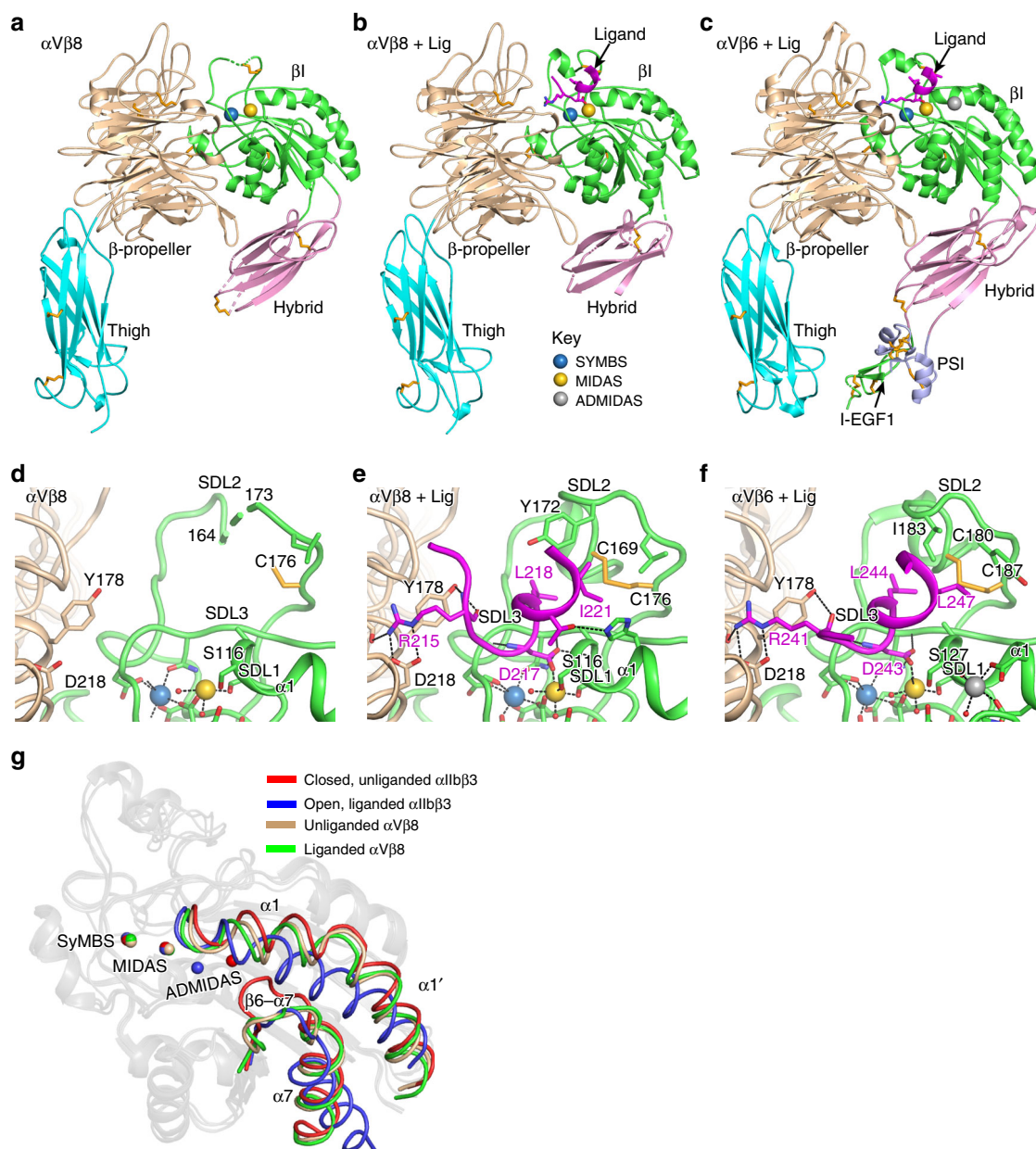
Fig. 2 αVβ8 headpiece structure and ligand-binding site. a–c Overall headpiece structures and d–f ligand-binding sites of αVβ8 ( a, d ), αVβ8 with ligand ( b, e ), and αVβ6 with ligand ( c, f ) 17 . The color scheme in d–f is the same as in a–c . In αVβ8 the PSI and EGF-1 domains are missing in electron density as are portions of the hybrid domain; shorter missing breaks in the hybrid domain are dashed. In all panels, structure representation in PyMol shows ribbon cartoon, key sidechains with oxygens in red and nitrogens in blue, disulfides in yellow, metals in the βI domain as spheres, and metal coordination bonds and key hydrogen bonds as dashed lines. Waters are shown as small red spheres. g βI domain regions that move in αIIbβ3 in typical integrins are compared to their counterparts in αVβ8 and shown in colored worm-like traces, while non-mobile regions are shown in gray ribbon cartoon. Metal ions are shown as spheres with the same color code as worm-like traces. Structures are closed, unliganded (PDB code 3T3P) and open, liganded (2VDR) αIIbβ3 and unliganded (chains A and B), and liganded (chains C and D) of αVβ8.
