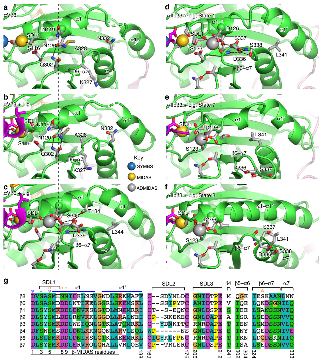
Fig. 3 Residues important in \beta domain allostery. a–f The mobile portion of the \beta I domain is shown in a unliganded \alpha V \beta 8, chain D; b liganded \alpha V \beta 8, chain B; c liganded \alpha V \beta 6 (4UM9, chain B); d liganded \alpha IIb \beta 3 in state 1 (3ZDY, chain D); e liganded \alpha IIb \beta 3 in state 7 (3ZDZ, chain B); and f liganded \alpha IIb \beta 3 in state 8 (2VDR, chain B). Structure representation is as in Fig. 2, except that sidechain carbons are in silver and mainchain carbons are in green. Vertical dashed lines mark the position of the \beta -MIDAS motif D8 C \alpha atom in \alpha IIb \beta 3 state 1 ( d ). g Sequences of all human integrin \beta I domains in regions that are important in ligand binding, shape shifting, or appear to have unusual residues in \beta 8. Residues with sidechain or mainchain coordination to the MIDAS or ADMIDAS in typical integrins are asterisked in blue and orange, respectively. \beta -MIDAS residue positions and \beta 8-subunit residue numbers are shown at the bottom.
