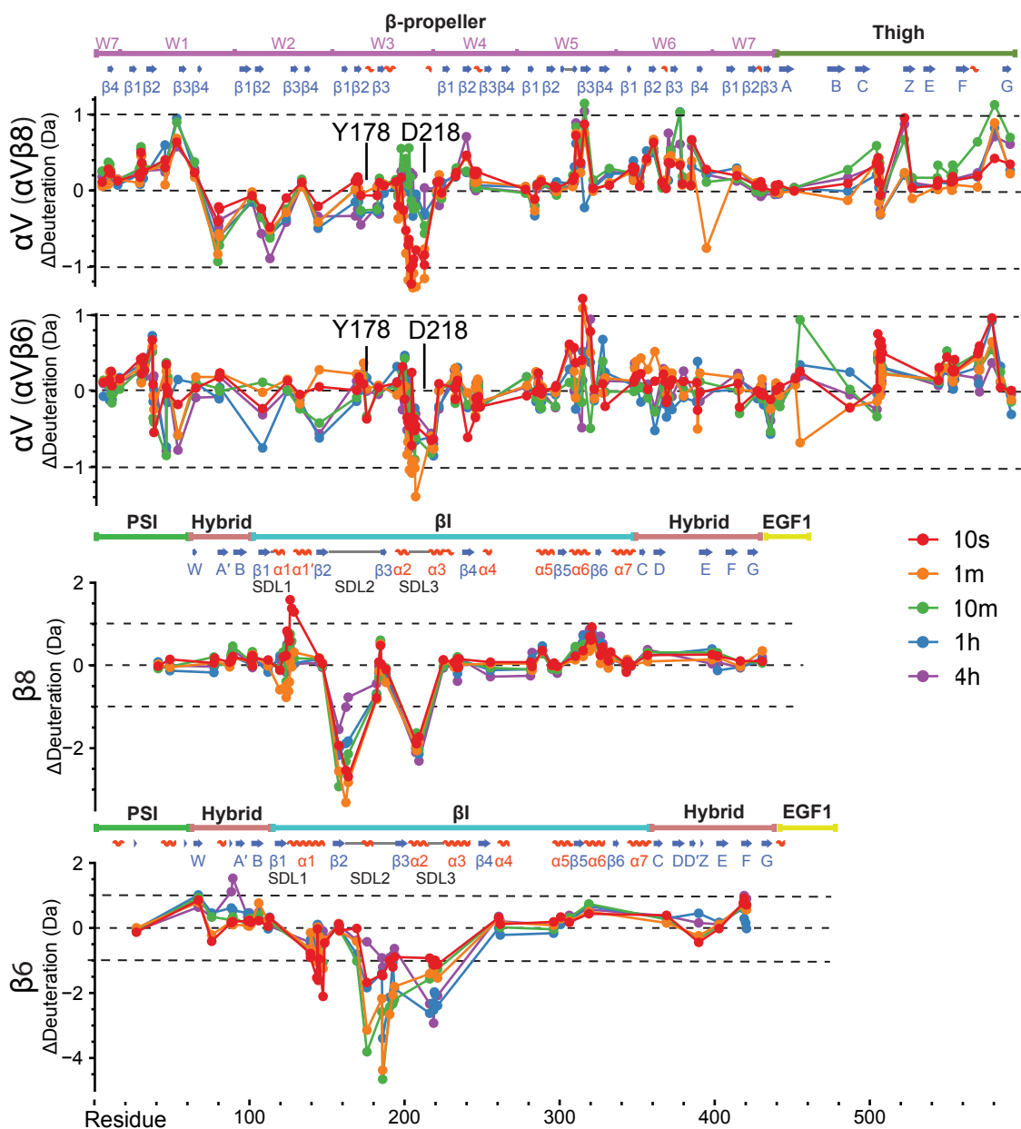
Supplementary Figure 2. Effect of ligand binding on hydrogen deuterium exchange. Difference in exchange for αVβ8 and αVβ6 (D incorporation for bound integrin - D incorporation for unbound integrin) is shown for each peptide plotted at the midpoint of its sequence position in the α or β-subunit. Differences greater than 1 Da (dashed lines) are considered meaningful.
