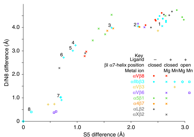
Fig. 4 Measurements from crystal structures of the relative positions of \beta -MIDAS S5 and D/N8 residues. Distances from an open conformation structure (integrin \alpha Ib \beta 3, PDB code 2VDR) of \beta -MIDAS S5 and D/N8 residues in liganded and unliganded integrin structures. Measurements show C \alpha atom—C \alpha atom distances. Numbers mark closed (1), open (8), and intermediate (2–7) ligand-bound states defined in a study in which ligand was soaked at different concentrations in Mg 2+ or Mn 2+ into crystals containing two independent copies of the closed \alpha Ib \beta 3 headpiece 21 . Crystal structures with missing \beta I domain metals or lacking deposited structure factors were not plotted. Representative \beta I domains from each integrin \beta -subunit were superimposed with Deep Align 36 . Each independent molecule in asymmetric units was then superimposed on the cognate \beta -subunit and distances were measured with PyMol to one-hundredth Å. The PDB code and chain ID of the plotted structure models listed as PDB/Chain ID in order of increasing S5 difference are 2VDR/B, 3ZE2/D, 4MMY/B, 5FFO/F, 4MMX/B, 5FFO/B, 4NEH/B, 3ZE0/B, 3ZE1/B, 3ZDZ/B, 3ZE2/B, 3ZE1/D, 3ZE0/D, 6OM2/B, 4NEN/B, 6OM2/D, 4WK4/B, 3VI4/B, 4WK2/B, 3ZDZ/D, 3VI4/D, 3ZDY/B, 4UM9/B, 3V4P/B, 3V4P/D, 4UM9/D, 6OM1/B, 5ES4/B, 6OM1/H, 6OM1/F, 3FCS/B, 4MMZ/B, 3FCS/D, 6OM1/D, 3ZDY/D, 3T3P/B, 3ZDX/B, 5E6U/B, 4WK0/B, 3T3P/D, 3ZDX/D, 5E6R/B, 5E6S/B, 4WJK/B, 3VI3/D, 3VI3/B.
