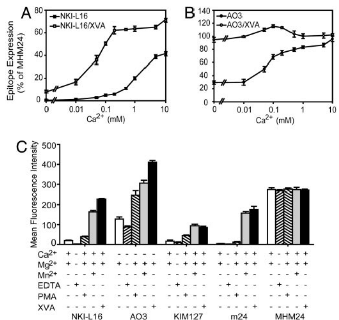
Fig. 1. Calcium and activation dependence of the NKI-L16 and AO3 epitopes. (A and B) \text{Ca}^{2+} dependence in the resting and extended conformations. K562 cells expressing WT \alpha_L\beta_2 were pretreated with EDTA and then washed twice with cation-depleted HBS. Binding of NKI-L16 and AO3 was measured in HBS containing 1 mM \text{Mg}^{2+} and varying concentrations of \text{Ca}^{2+} , with or without 1 \mu M XVA143 to induce extension. (C) Preferential binding to activation epitopes. K562 transfectants pretreated as in A and B were incubated with primary mAbs in HBS in the presence of 0.2 mM \text{Ca}^{2+} , 1 mM \text{Mg}^{2+} , 2 mM \text{Mn}^{2+} , 1 \mu M PMA, and 1 \mu M XVA143 for 30 min at 37°C. Cells were washed and incubated with FITC-labeled second Ab for 15 min at 4°C. Epitope expression was measured as specific mean fluorescence intensity in C (after subtraction of control X63 intensity) or further quantitated as the percentage of fluorescence intensity with MHM24 mAb to the \alpha_L I domain in A and B. Results are the mean \pm SD of three independent experiments.
