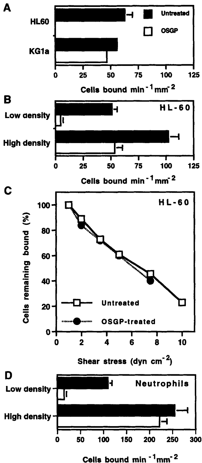
Figure 5. Effect of OSGP treatment on tethering to L-selectin chimera. (A) HL-60 and KG1a cells treated with or without OSGP were allowed to tether at a wall shear stress of 1.0 dyn/cm 2 to L-selectin chimera plated at 2 μg/ml on protein A. Data are mean ± range of two observations. (B) OSGP-treated and untreated HL-60 cells were allowed to tether at a wall shear stress of 1.0 dyn/cm 2 to L-selectin chimera plated at 2 μg/ml ( Low density ) or 10 μg/ml ( High density ). Data are mean ± range of two observations. (C) OSGP-treated and untreated HL-60 cells accumulated on high density L-selectin chimera were subjected to graded increases in wall shear stress every 20 s and the percentage of cells remaining bound at each shear was determined. (D)
